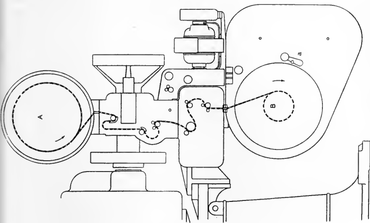
FIG. 3. Standard 2000-ft reels for ordinary sound and picture projection.
